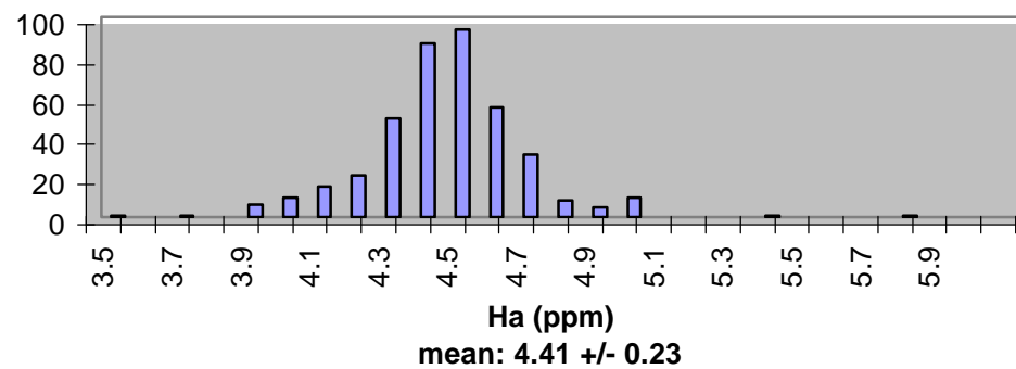
Alpha Helix D CO
