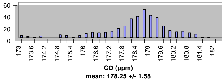
Alpha Helix L CO
