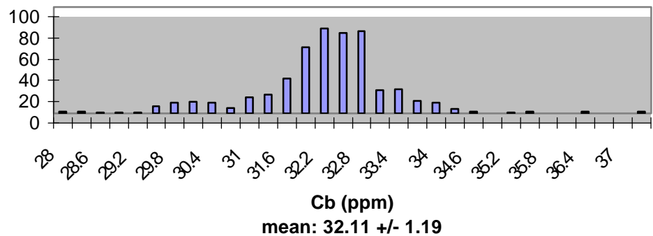
Alpha Helix K Cb
