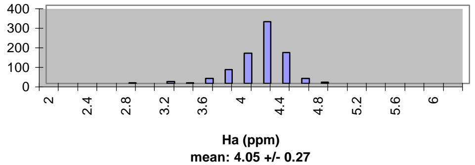
Alpha Helix A CO
