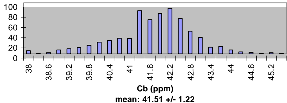
Alpha Helix L Cb
