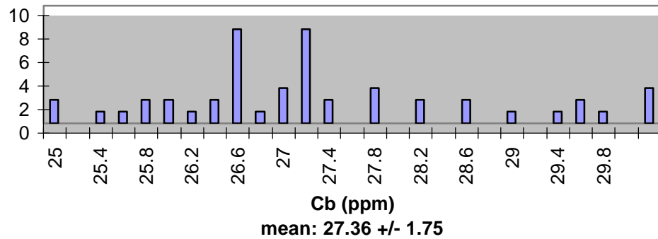
Alpha Helix B Cb
