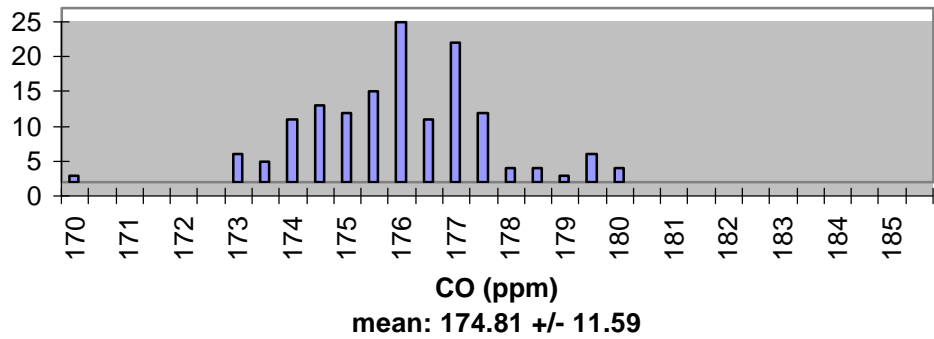
Alpha Helix G CO
