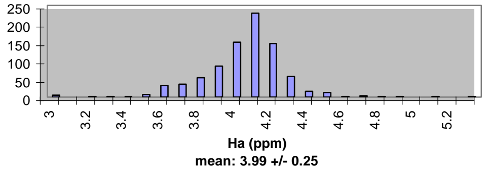
Alpha Helix E CO
