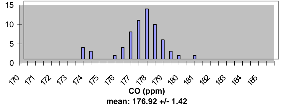
Alpha Helix H CO
