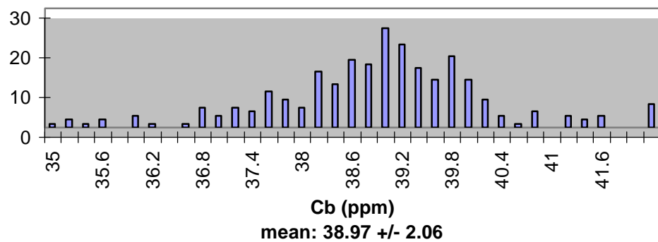
Alpha Helix F Cb
