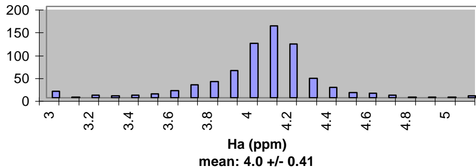
Alpha Helix K CO
