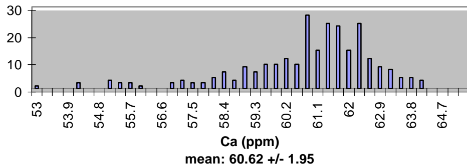
Alpha Helix F Cb
