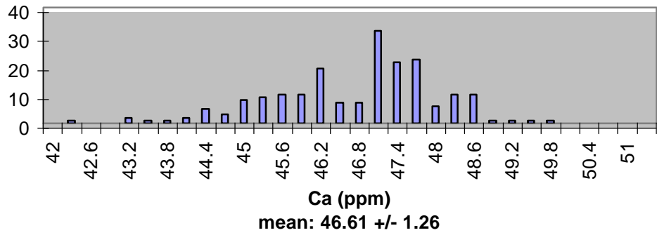
Alpha Helix G CO
