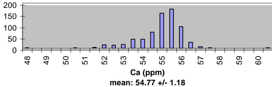
Alpha Helix A Ca
